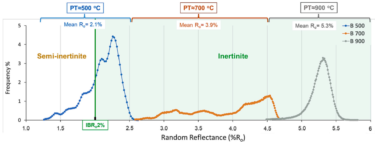
Fig. 13. The R_0 frequency distribution histograms depict three bamboo biochar samples created at distinct production temperatures (PT): 500, 700, and 900 °C (heating rate of 10 °C/min). Findings reveal a rise in both range and mean R_0 values as the temperature increases. Specifically, 85% of the biochar from 500 °C, and the entire range from 700 °C and 900 °C, surpass the Inertinite Benchmark (IBR 0 2%).
